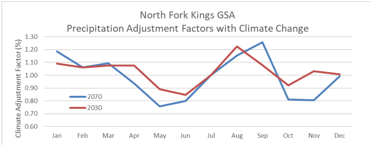
Figure VI-3. Estimated Precipitation Impacts in NFKGSA with Climate Change
