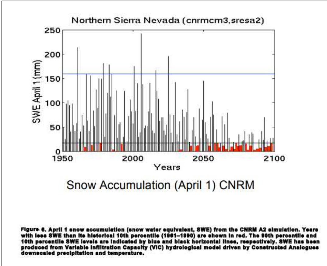
Figure VI-1. Projected Sierra Nevada Snowpack 1
