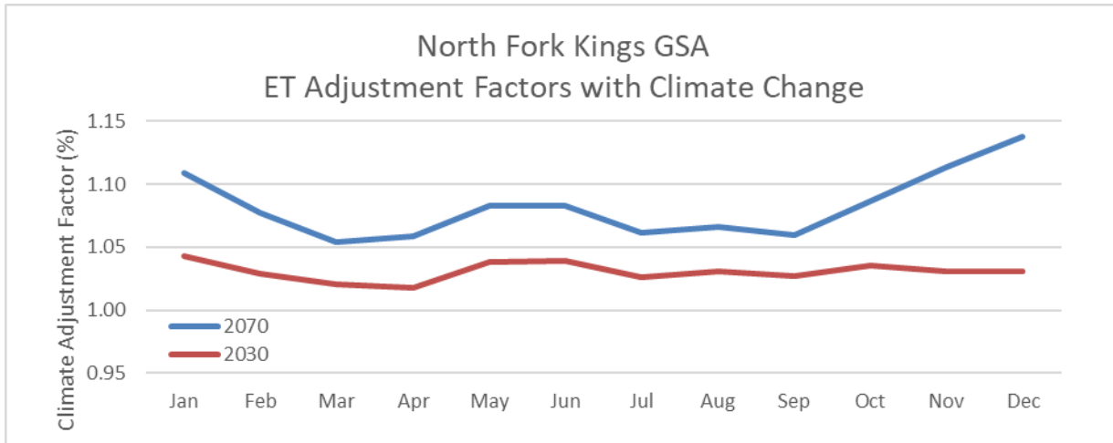
Figure VI-4. DWR Evapotranspiration Adjustment Factors with Climate Change in NFKGSA
