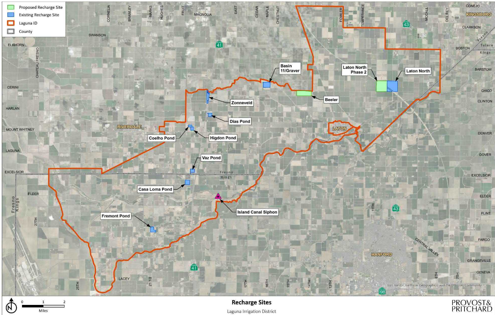
Figure II-3. District Recharge Facilities and Proposed Projects
